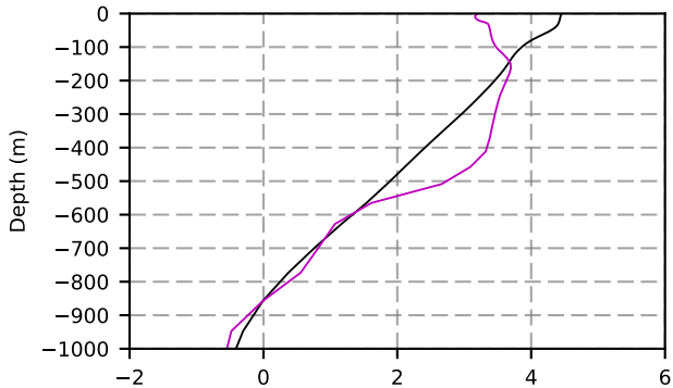
1984 mean temperature @ moor GIN seas box
