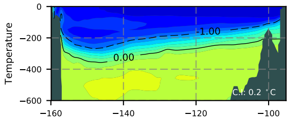
ERA01NEM405MLD / Beaufort Section 1982
