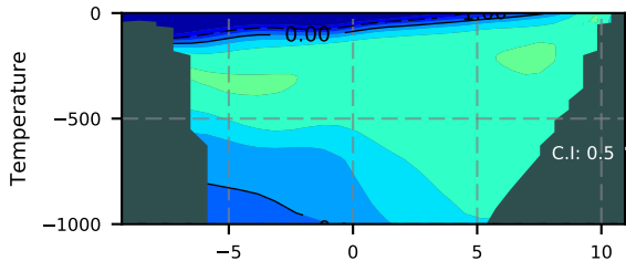
ERA01NEM405MLD / FramS Section 1980
