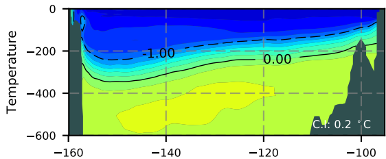
ERA01NEM405NMP / Beaufort Section 1987
