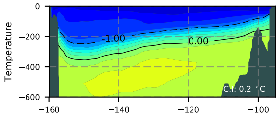
ERA01NEM405NMP / Beaufort Section 1988
