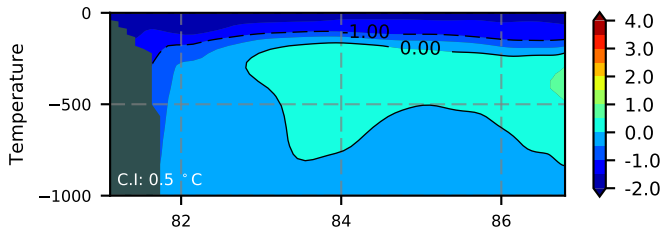
ERA01NEM405NMP / Kara Section 1986
