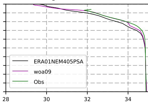
1981 mean Salinity @ moor Arctic B box
