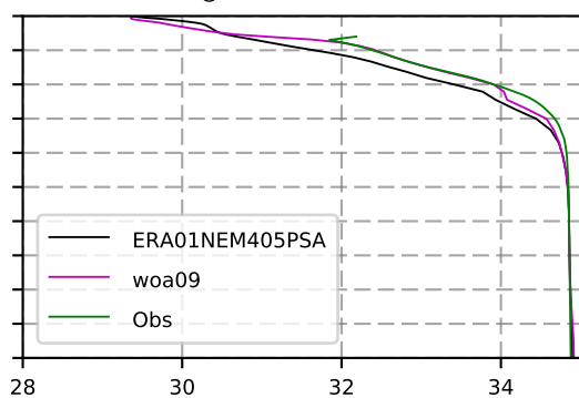
1987 mean Salinity @ moor Arctic B box
