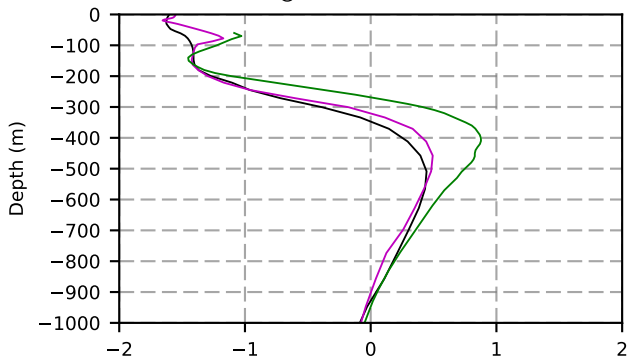
1987 mean temperature @ moor Arctic B box
