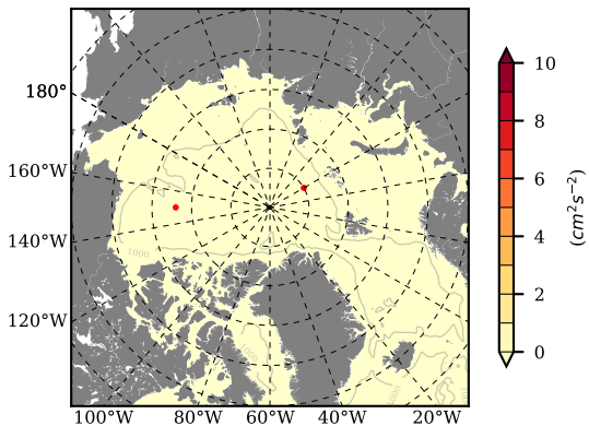
ERA01NEM405PSC mean EKE @ 0 m over 1991
