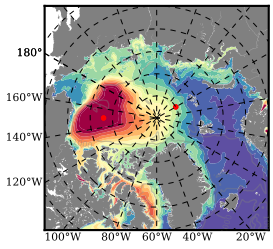
ERA01NEM405PSC mean FWC (m) over 2009
