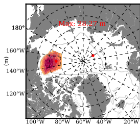
Mean FWC (m) from BG Obs Sys. (Proshutinsky et al. GRL2018) over year 2014
