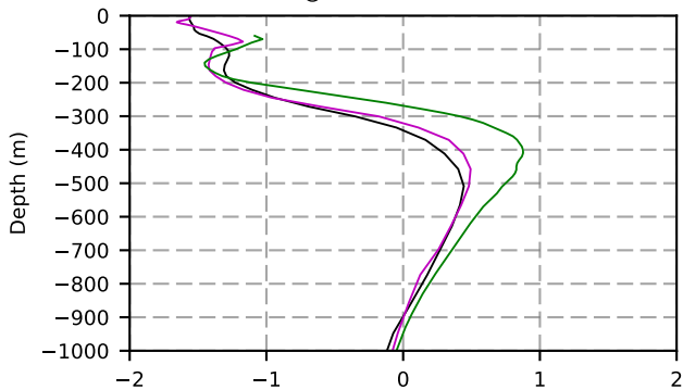
1990 mean temperature @ moor Arctic B box
