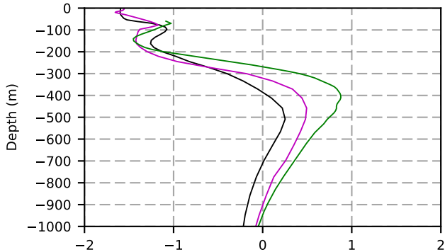
1994 mean temperature @ moor Arctic B box
