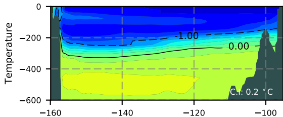
ERA01NEM405PSC / Beaufort Section 1979
