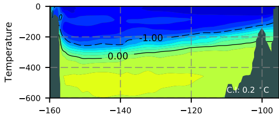
ERA01NEM405PSC / Beaufort Section 1980
