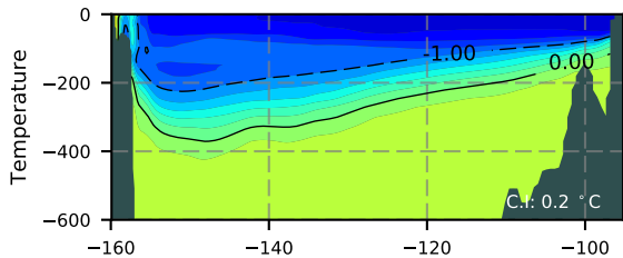
ERA01NEM405PSC / Beaufort Section 1997
