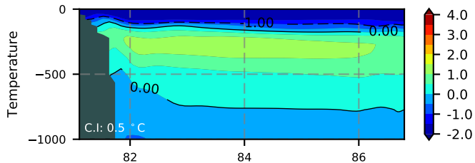
ERA01NEM405PSC / Kara Section 1979
