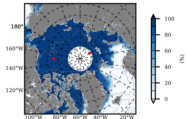
NSIDC mean SICON m09 1979
