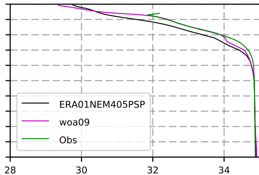
1989 mean Salinity @ moor Arctic B box
