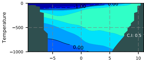
ERA01NEM405QNS / FramS Section 1986
