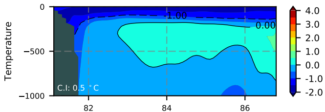
ERA01NEM405QNS / Kara Section 1985
