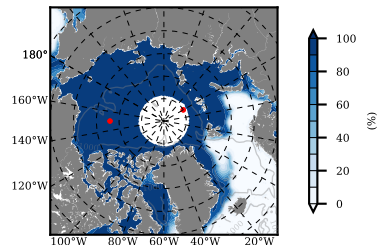
NSIDC mean SICON m09 1987
