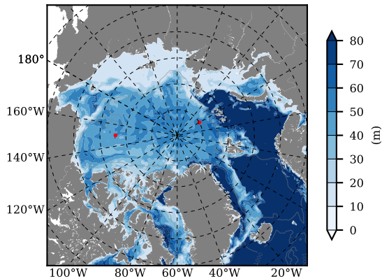
ERA01NEM405QTI mean MLD01 over 1983 m03
