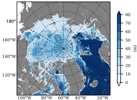
ERA01NEM405QTI mean MLD01 over 1987 m03
