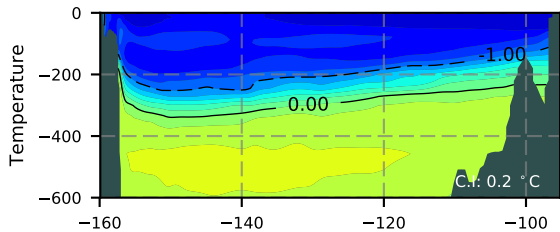
ERA01NEM405QTI / Beaufort Section 1980
