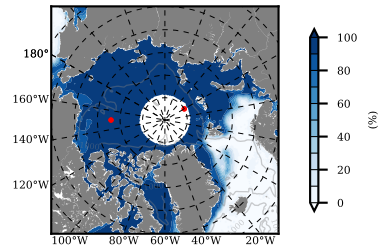
NSIDC mean SICON m09 1981
