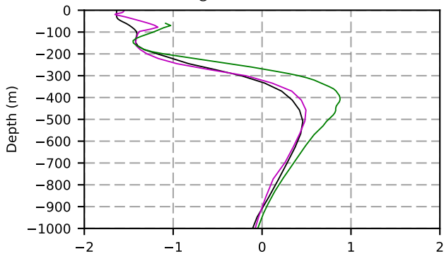
1986 mean temperature @ moor Arctic B box
