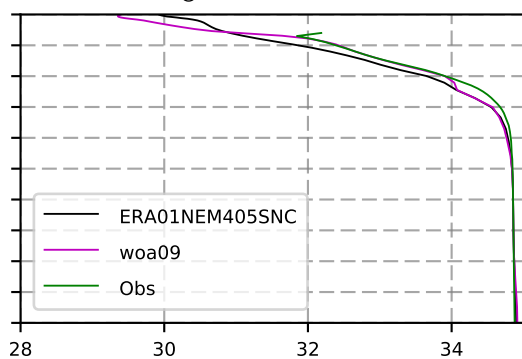
1986 mean Salinity @ moor Arctic B box
