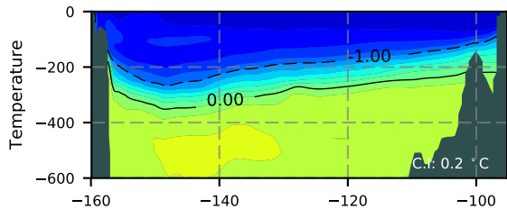
ERA01NEM405SNC / Beaufort Section 1982
