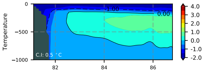
ERA01NEM405SNC / Kara Section 1983
