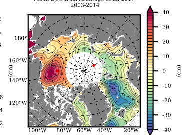
Mean DOT from Armitage et al. 2017 2003-2014
