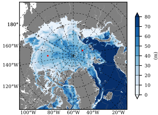
ERA01NEM405SNO mean MLD01 over 1990 m03
