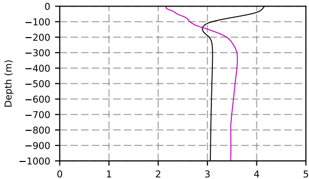
1983 mean temperature @ moor BRAVO box
