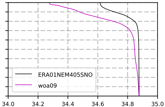
1983 mean Salinity @ moor BRAVO box
