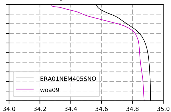
1987 mean Salinity @ moor BRAVO box
