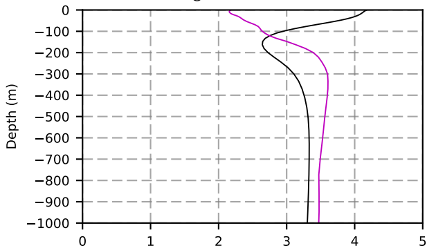
1987 mean temperature @ moor BRAVO box
