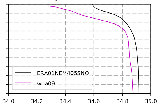
1990 mean Salinity @ moor BRAVO box
