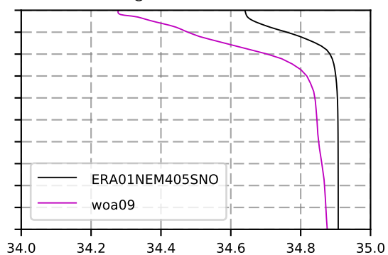
1991 mean Salinity @ moor BRAVO box
