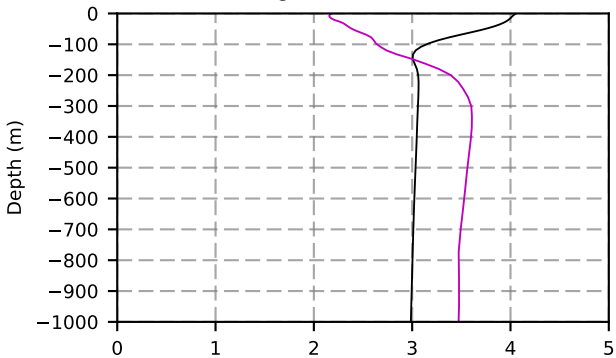
1992 mean temperature @ moor BRAVO box
