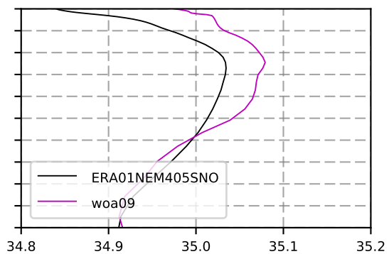
1988 mean Salinity @ moor GIN seas box
