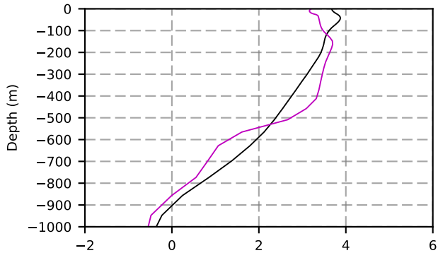
1988 mean temperature @ moor GIN seas box
