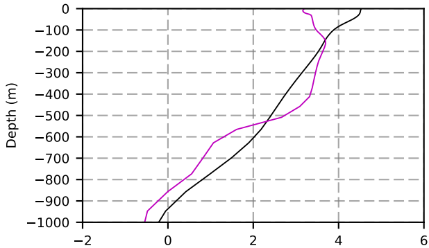
1993 mean temperature @ moor GIN seas box
