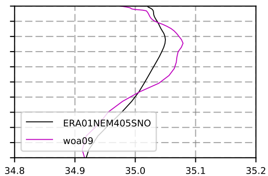
1993 mean Salinity @ moor GIN seas box
