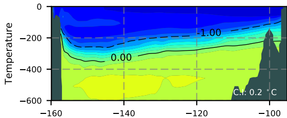
ERA01NEM405SNO / Beaufort Section 1981
