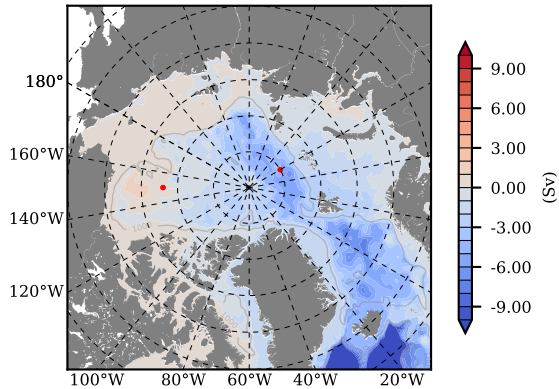
mean PSI over 1987
