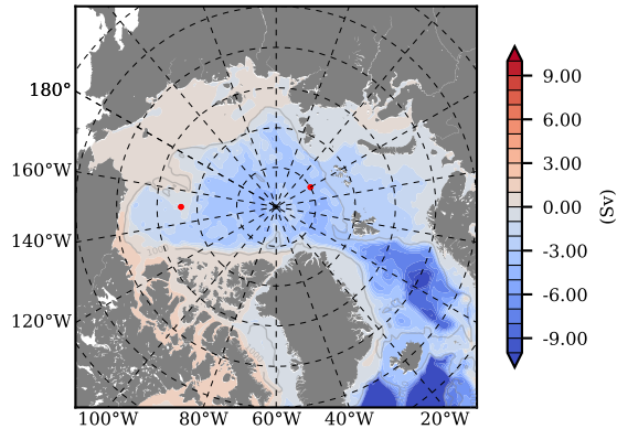
mean PSI over 2000
