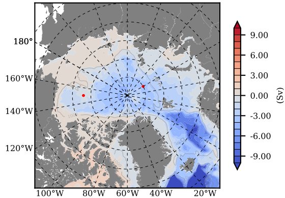
mean PSI over 2002
