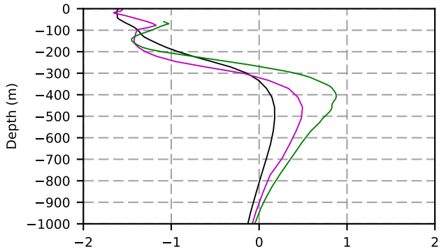
2004 mean temperature @ moor Arctic B box
