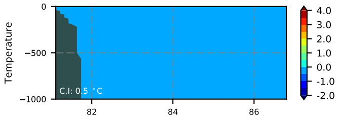
NEMO420 / Kara Section 1979
