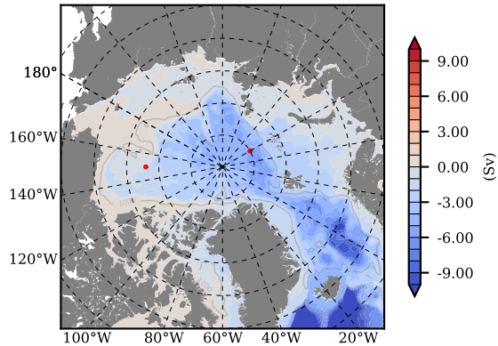
mean PSI over 1994
