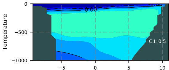
NEMO420IRW / FramS Section 1981
