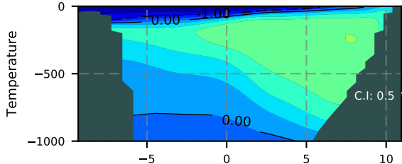
NEMO420IRW / FramS Section 1985
