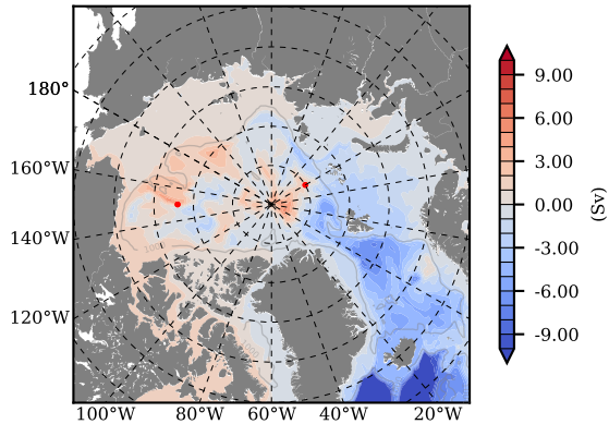
mean PSI over 1979
