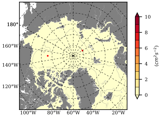
NEMO420WND mean EKE @ 0 m over 1986
