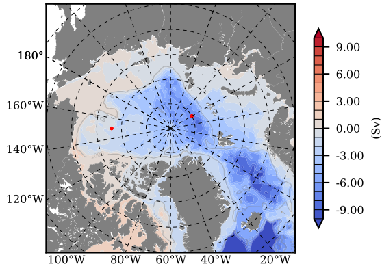
mean PSI over 1989
